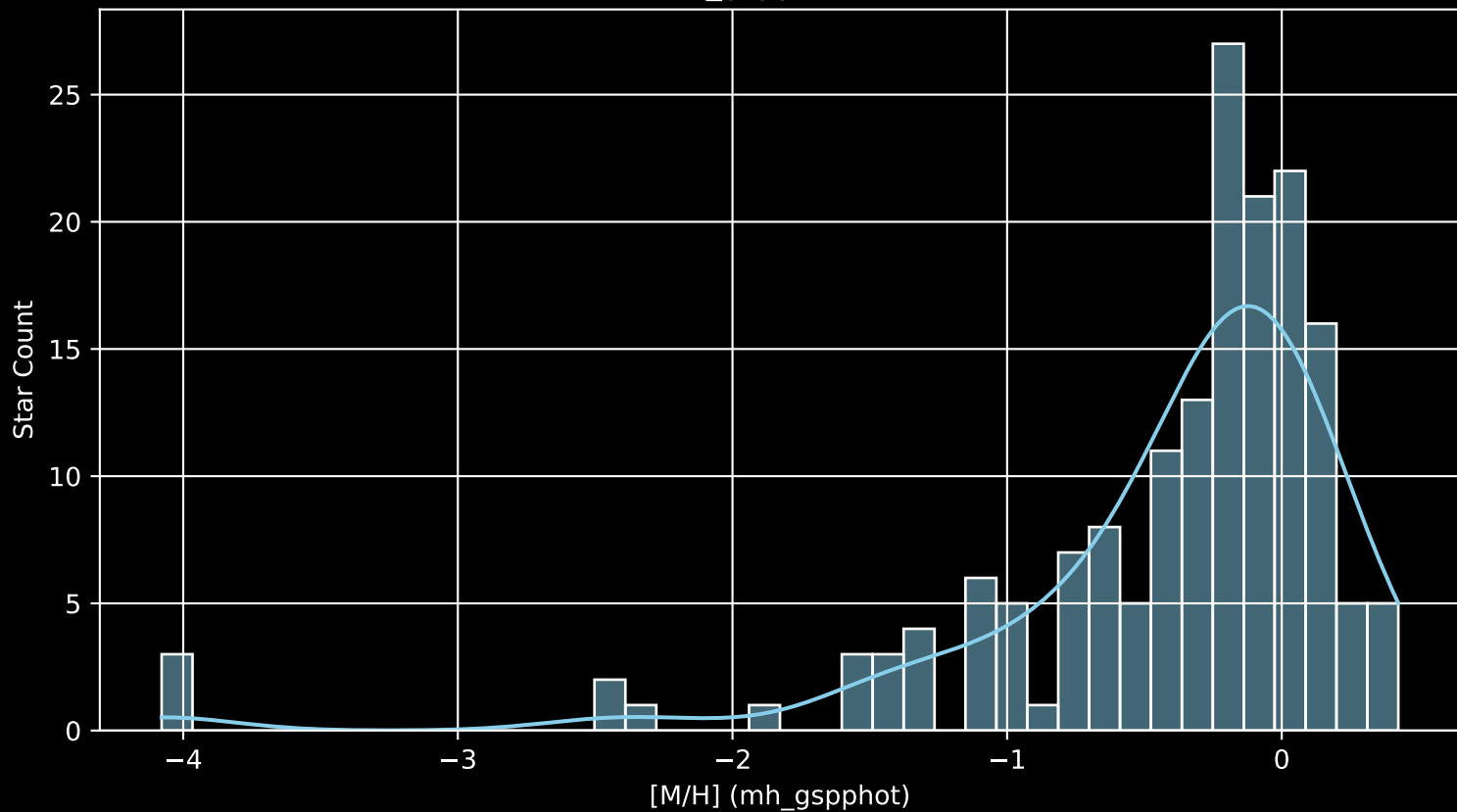
APOGEE DR17 Field: [TAUL1536 [M/H] (mh_gspphot) (n= 169)
