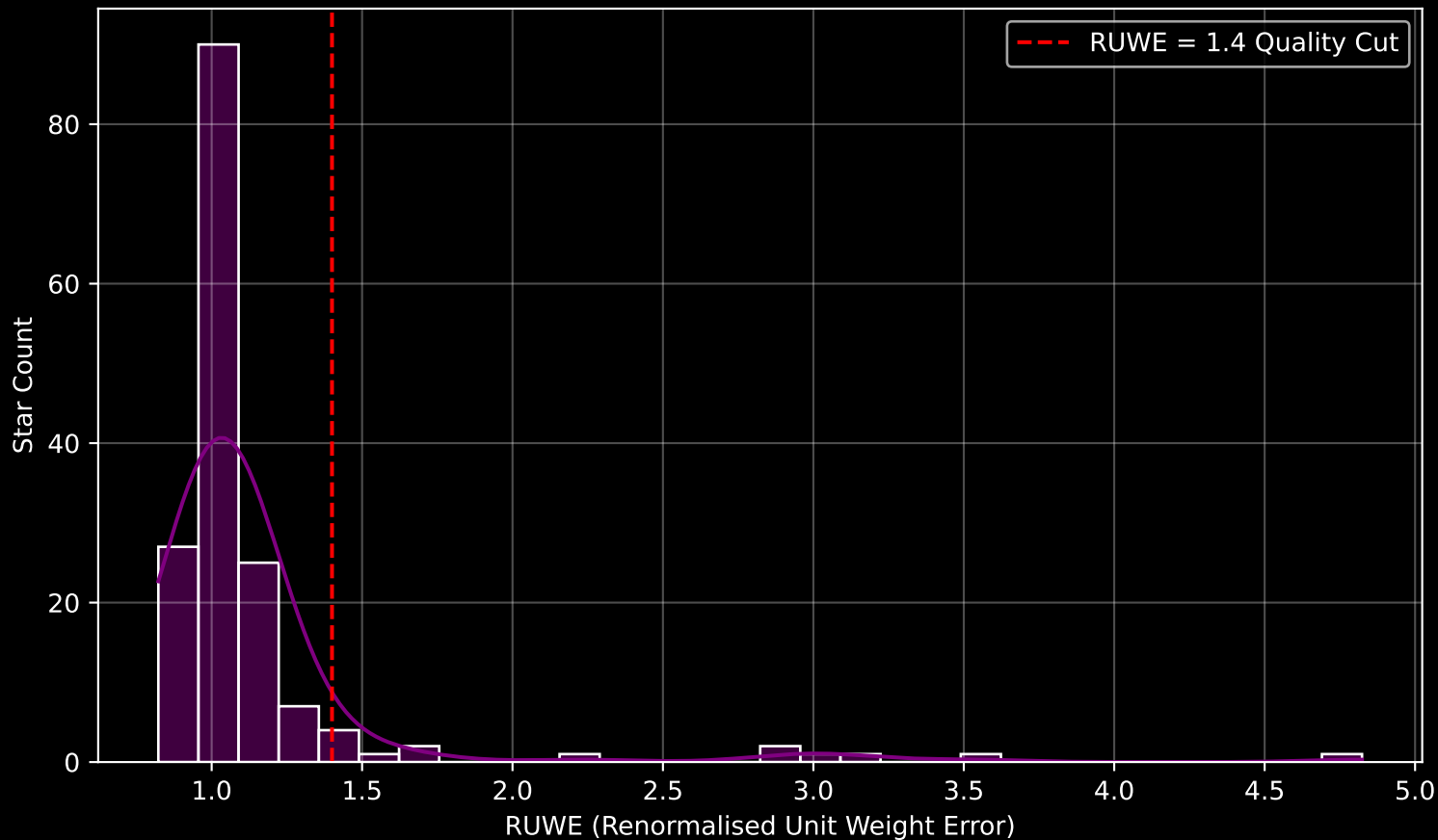
GAPOGEE DR17 Field [TAUL1536] RUWE Distribution (n= 163)
