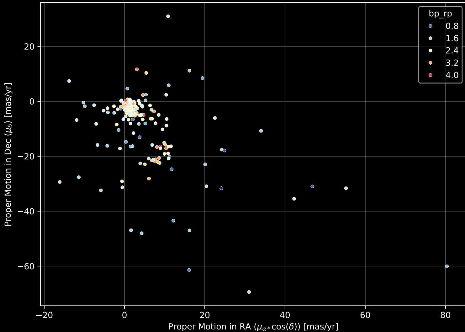
APOGEE DR17 Field: [TAUL1536] Proper Motion Diagram (n= 170)
