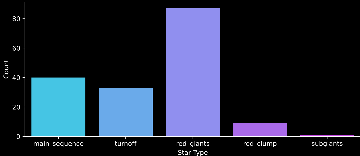
APOGEE DR17 Field: [TAUL1536] Count plot of Star Type
