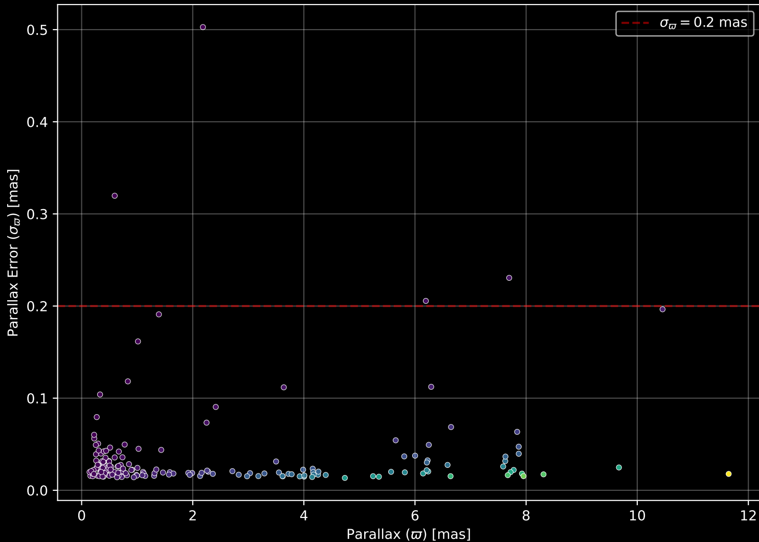
APOGEE DR17 Field: [TAUL1536] Parallax Quality (n= 170)
